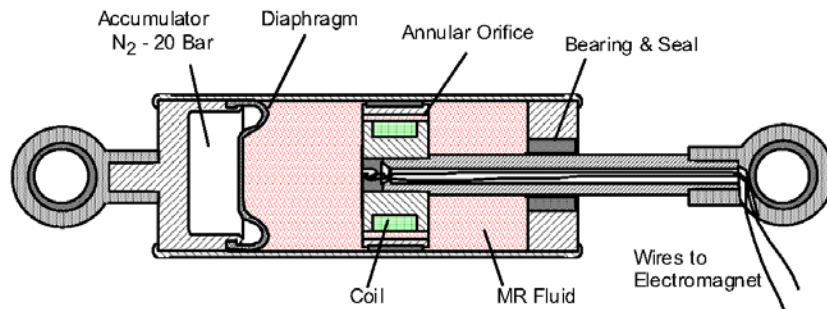
Figure 6: Sketch of a monotube MR damper for seat suspension from Lord [29]
